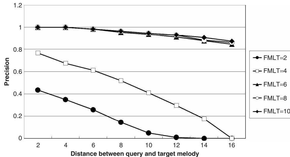
Fig. 20. Precision of the frequent melody suffix tree index with various values of FMT and various distances between queries and their corresponding target music (BST = 2, 3000 songs, query length = 15 s).
