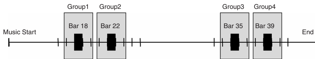
Fig. 6. A set of initial groups constructed from the bars of Table 1 whose rank values are 1.
