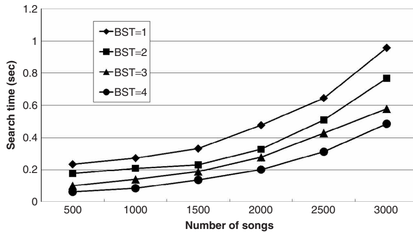
Fig. 14. Search time of the frequent melody suffix tree index when the value of BST is 1, 2, 3 and 4, respectively (FMLT = 6, query length = 15 s).
