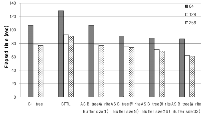
Fig. 11. Elapsed time of update operations.
