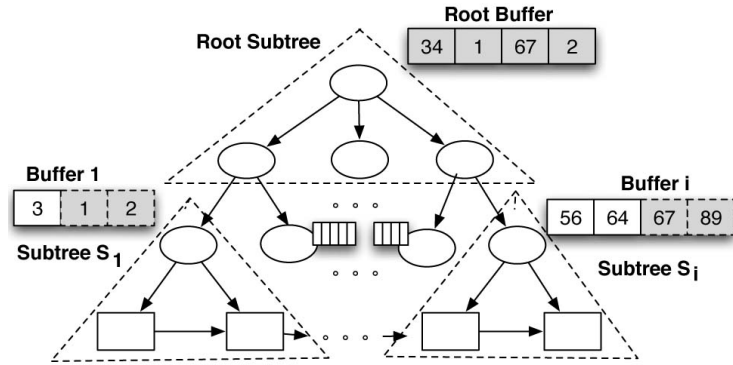
Fig. 3. (b) System architecture of LA-tree [20].
