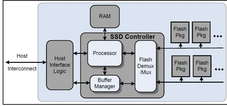
Fig. 2. SSD logic components [1].
