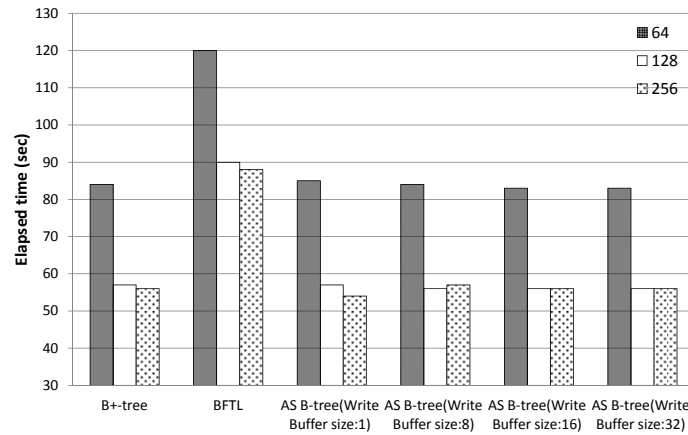
Fig. 10. Elapsed time of search.
