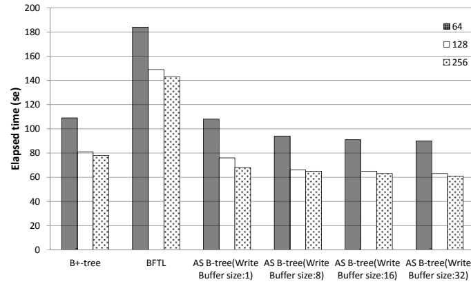
Fig. 12. Elapsed time of delete operations.
