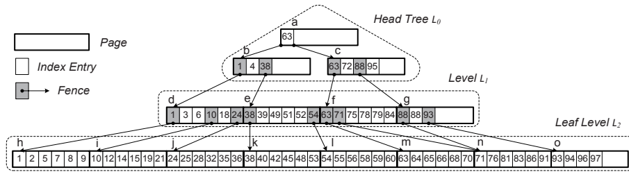
Fig. 3. (c) System architecture of FD-tree [19].
